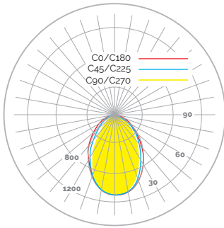
12W 60° with Micro Louvre
